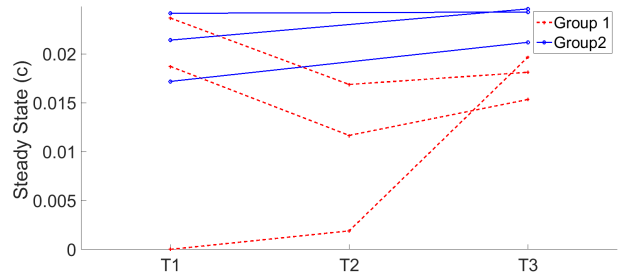
Fig. 8: Steady state value of error
