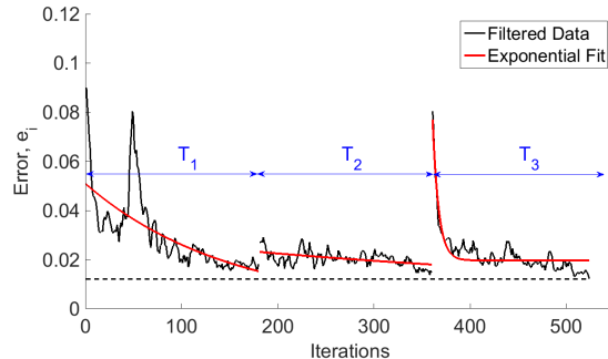
Fig. 3: The evolution of error for all tasks performed by Subject-3 from Group-1.
