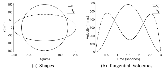
Fig. 1: (a) Shapes in XY coordinates and (b) tangential velocity profiles, used to define the different tasks.
