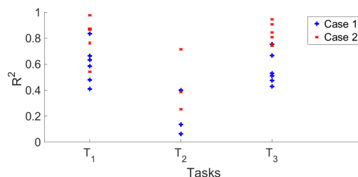
Fig. 5: R^2 values for Case-1 and Case-2
