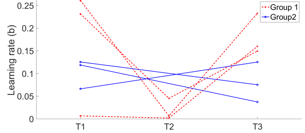
Fig. 7: Learning rate of all tasks
