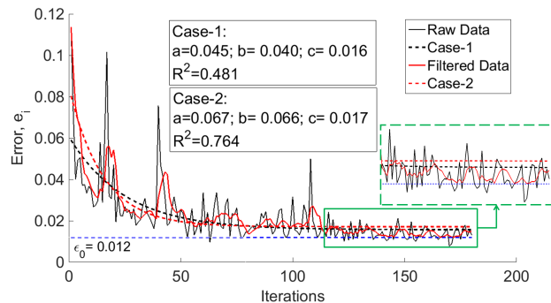
Fig. 4: Curve fitting : Subject-6, Task, T_1
