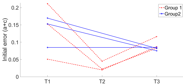
Fig. 6: Initial error of all tasks T_1, T_2 and T_3
